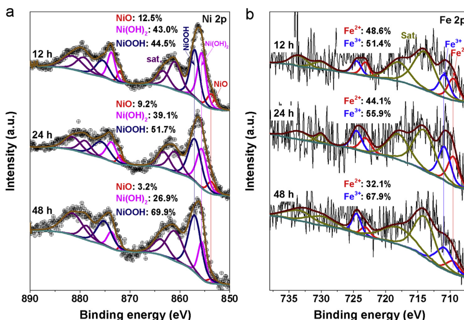
Fig. 2 – High-resolution XPS spectra of (a) Ni 2p and (b) Fe 2p from FeOOH–NiOOH/NF-12 h, –24 h and –48 h, respectively.
