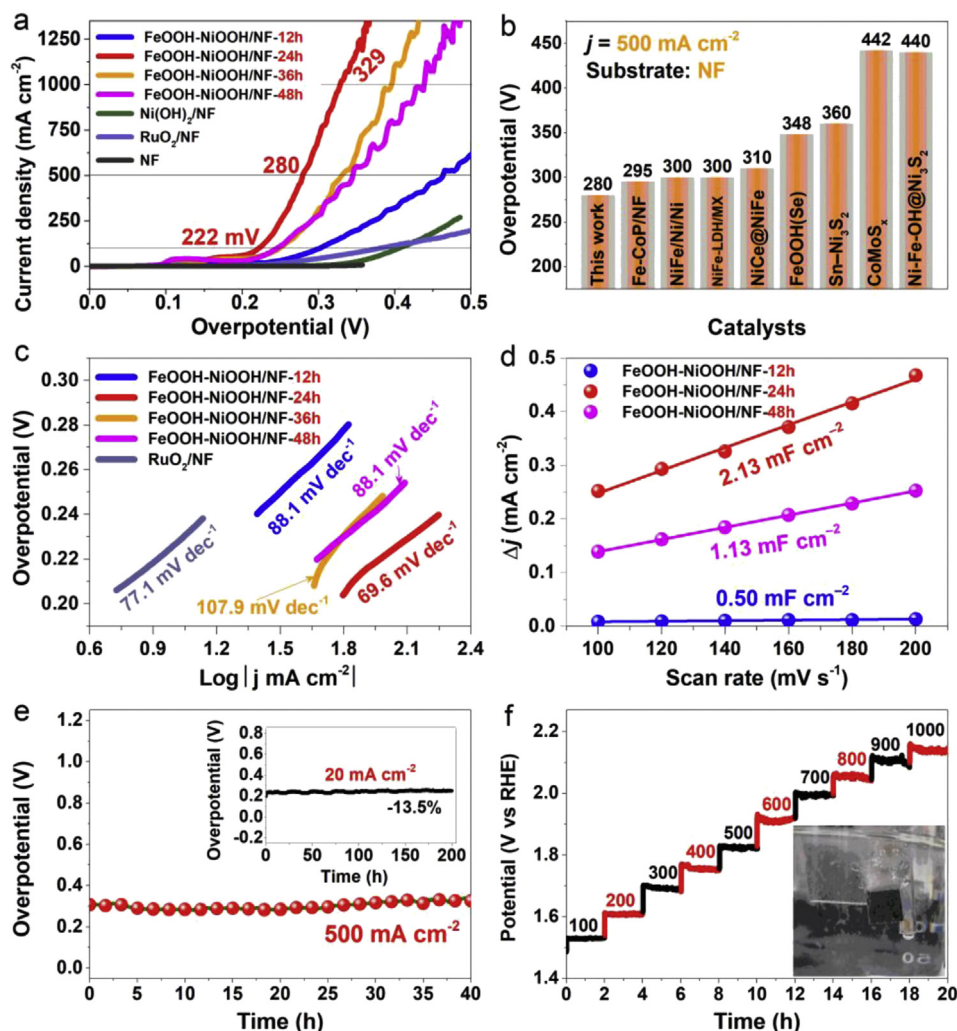
Fig. 3 – OER catalytic performance of different catalysts in 1.0 M KOH. (a) LSV curves with a scan rate of 2 mV s -1 . (b) Comparison of OER activities among the published catalysts at a current density of 500 mA cm -2 . (c) Tafel slopes calculated from LSV curves. (d) The summarized double-layer capacitance ( C_{dl} ) of different catalysts. (e) Chronoamperometric test of FeOOH–NiOOH/NF-24 h catalyst at 500 mA cm -2 for 40 h (Inset: 20 mA cm -2 for 200 h). (f) Multi-step chronopotentiometric curves of FeOOH–NiOOH/NF-24 h from 100 to 1000 mA cm -2 with an increment of 100 mA cm -2 per 2 h (Inset: test photo).
